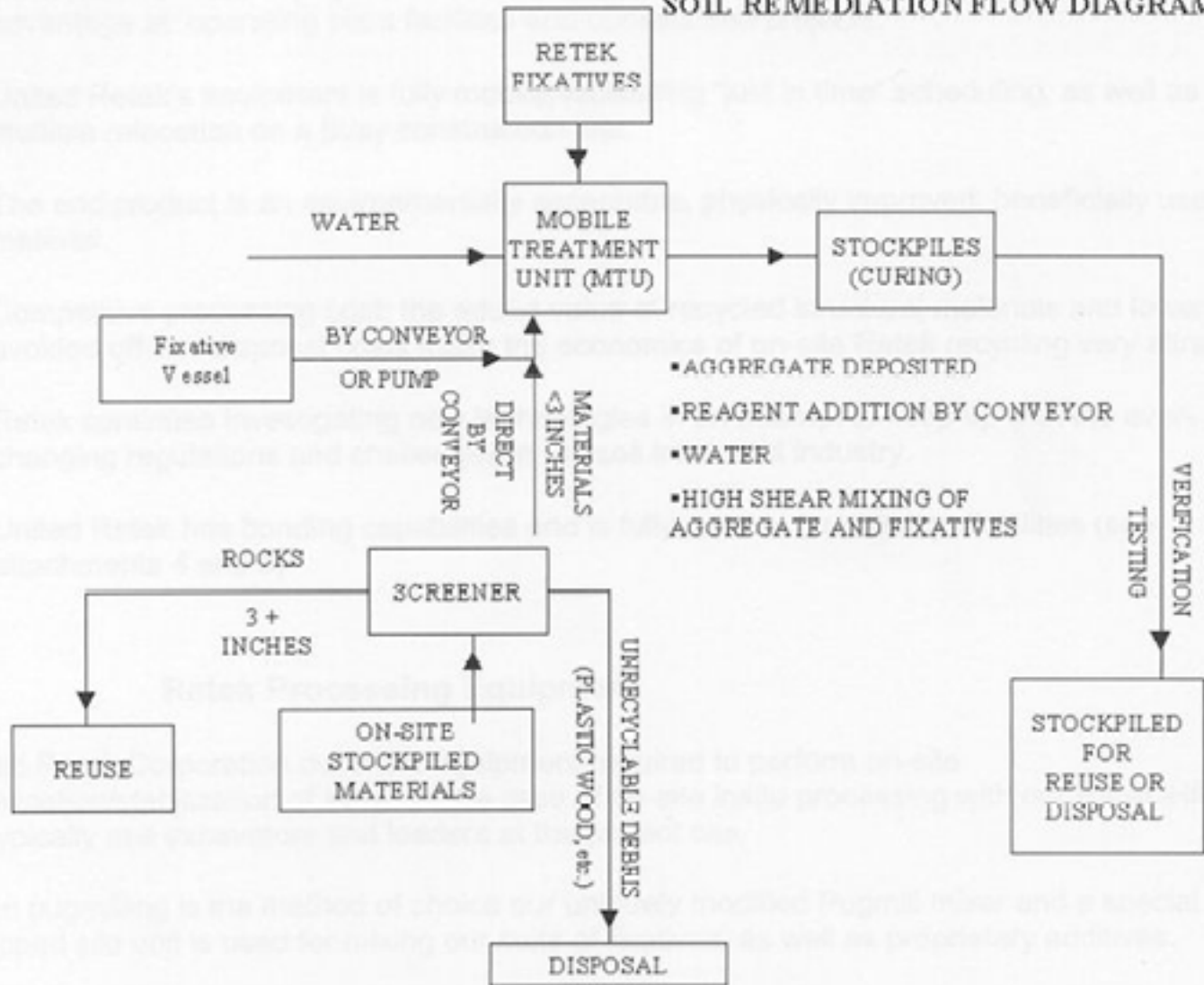
Figure 1 Typical Petroleum Contaminated Soil Remediation
